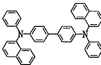
NPD
