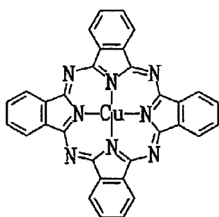
CuPC
