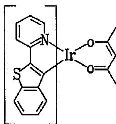
(btp)_2Ir(acac)
